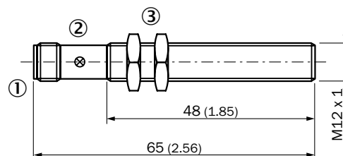
All dimensions in mm (inch)
