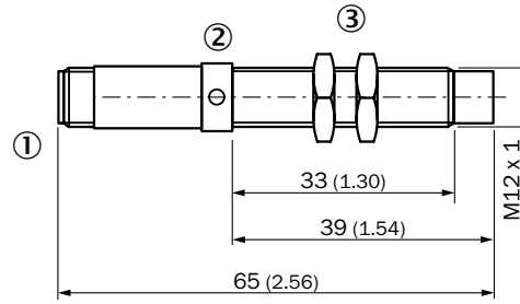
IMF12-xxNxxxxxx, M12, non-flush
